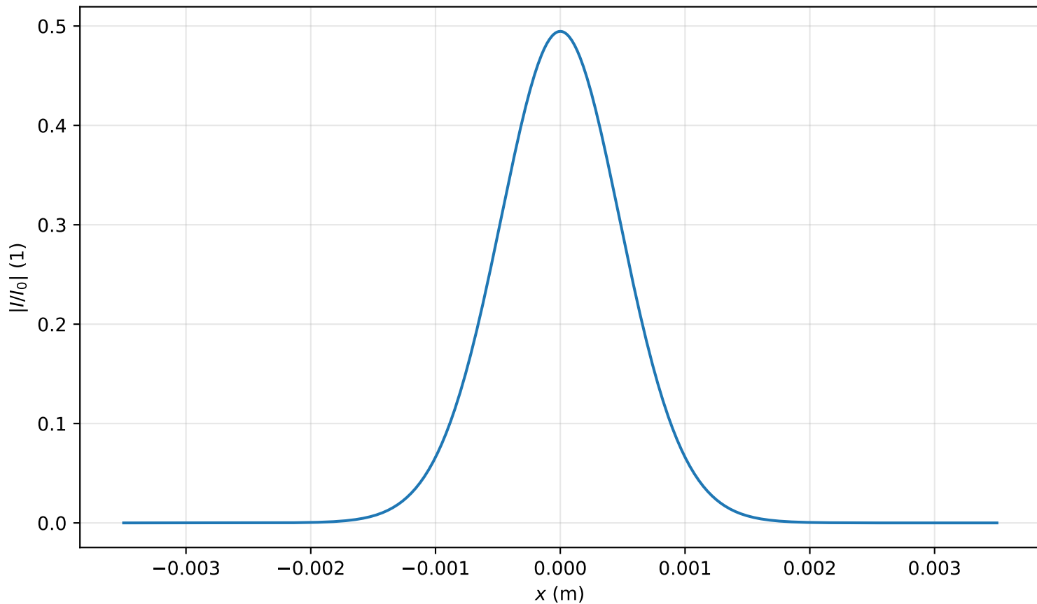
Intensity profile I(x, y = 0, z = 2.388m)/I_0 , P_{in}=0.2P_{cr} , artificial time
